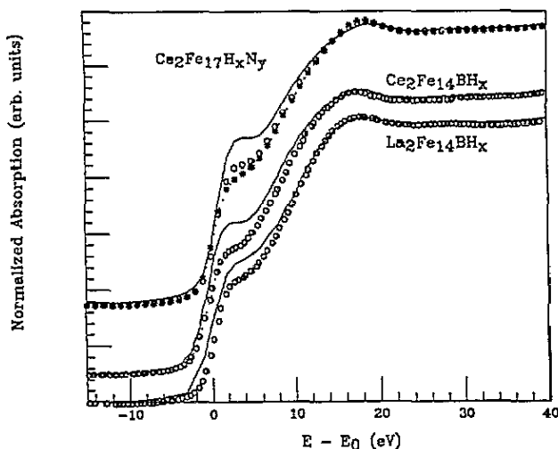
Figure 1. Comparison between the experimental XANES spectra at the Fe K edge in the case of \text{La}_2\text{Fe}_{14}\text{B} , \text{Ce}_2\text{Fe}_{14}\text{B} and \text{Ce}_2\text{Fe}_{17} (solid) and their hydride derivatives. In the case of \text{Ce}_2\text{Fe}_{17} also the nitride \text{Ce}_2\text{Fe}_{17}\text{N}_y is shown (*).
