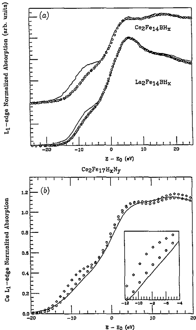
Figure 3. Comparison between the experimental XANES spectra at the rare earth L_1 edge in the case of (a) \text{La}_2\text{Fe}_{14}\text{B} and \text{Ce}_2\text{Fe}_{14}\text{B} (solid) and their hydride derivatives (dots); (b) \text{Ce}_2\text{Fe}_{17} (○), \text{Ce}_2\text{Fe}_{17}\text{H}_x (dots) and \text{Ce}_2\text{Fe}_{17}\text{N}_x (solid). The inset reports the differences of the near edge region for the hydride and nitride derivatives.
